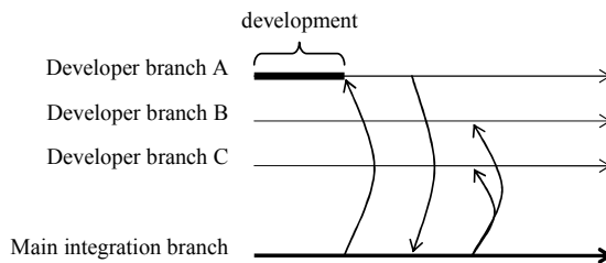
Figure 1: copy/merge integration model [15]
